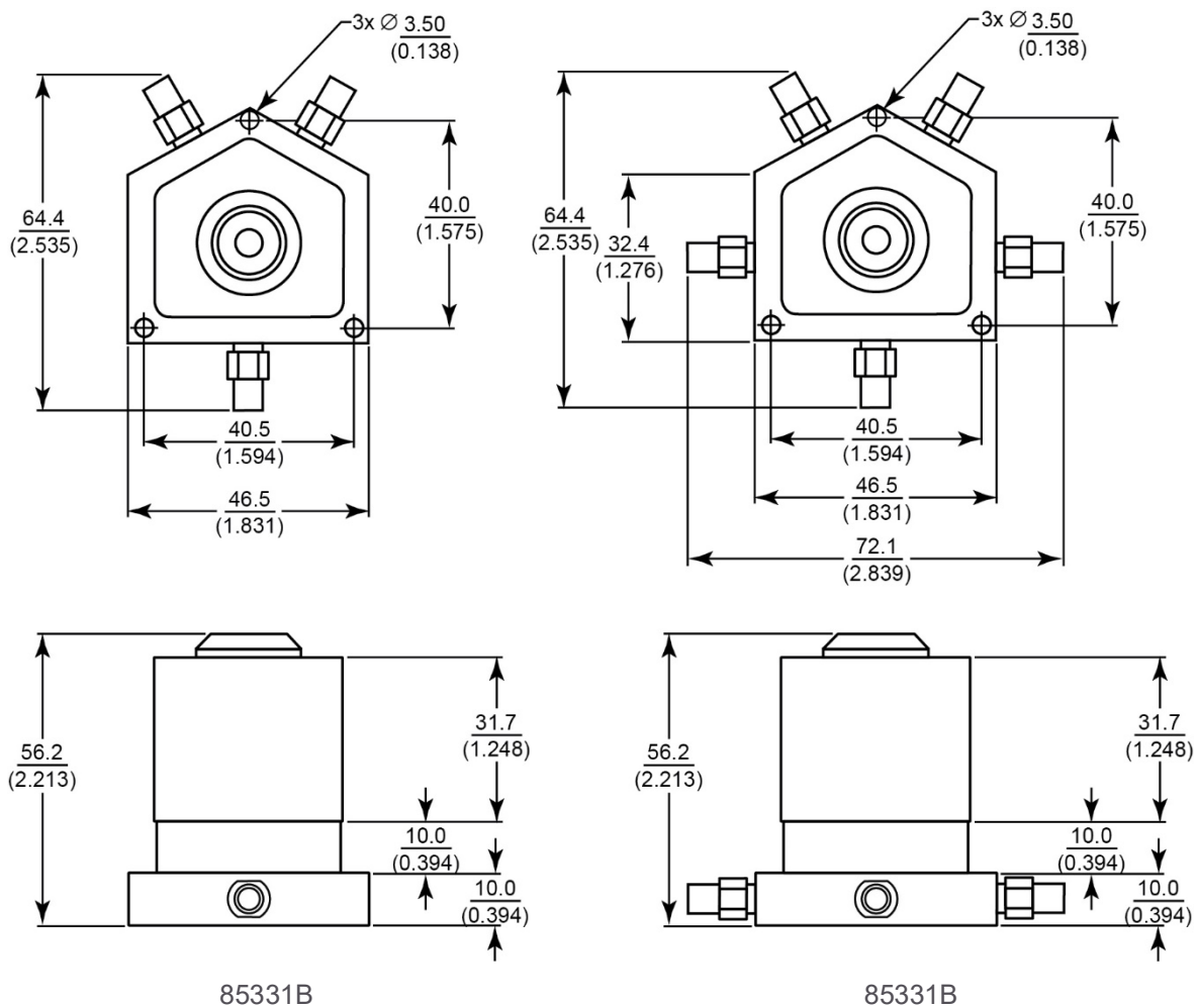
Figure 4. Product mechanical outline. Dimensions are in mm (inches) nominal, unless otherwise specified.
