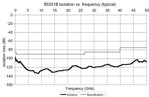
Figure 9. 85331B isolation vs. frequency (typical)
