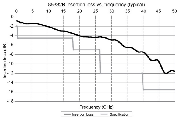
Figure 10. 85332B insertion loss vs. frequency (typical)
