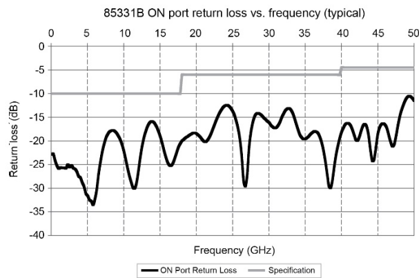
Figure 7. 85331B ON port return loss vs. frequency (typical)
