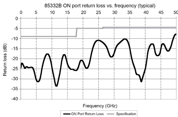
Figure 12. 85332B ON port return loss vs. frequency (typical)
