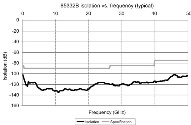
Figure 14. 85332B isolation vs. frequency (typical)
