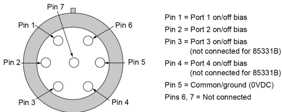
Figure 3. Bias connector pin locations
