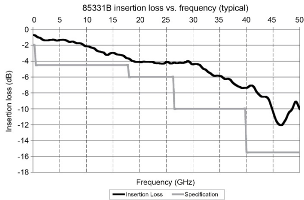
Figure 5. 85331B insertion loss vs. frequency (typical)
