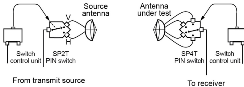
Figure 1. A typical multiple-channel, multiple frequency system configuration
