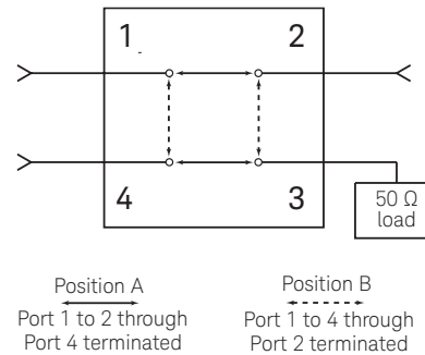
Figure 5. SPDT terminated
