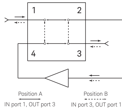
Figure 4. Signal reversal
