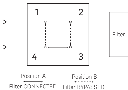
Figure 3. Drop-out switch
