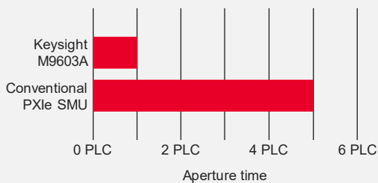
Figure 3. Aperture time required to achieve 400 fArms current measurement noise
