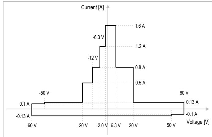
Figure 7. DC voltage and current output capability (With mode for the chassis supporting 4 A backplane pin current capacity for 12 V rail.)
