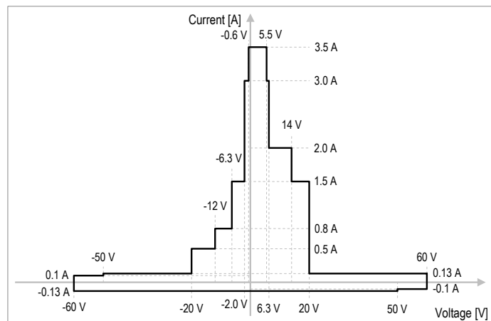
Figure 6. DC voltage and current output capability (With mode for the chassis supporting 6 A backplane pin current capacity for 12 V rail.)
