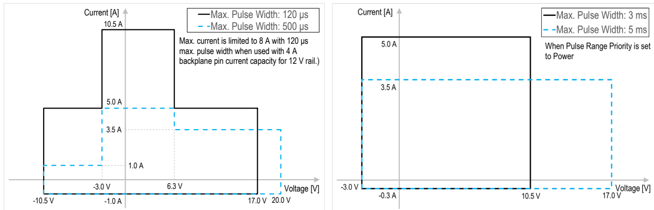
Figure 8. Pulsed voltage and current output capability
